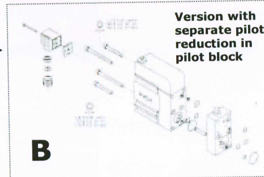
Replacement (PVE inclusive Intermediate plate)
